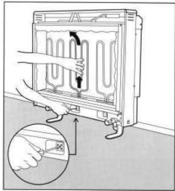
Figura 10 a - ACE 405 / 805 (A) / 1205 (A) / 1605 (A)
