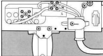
Figura 11 a - ACE 405 / 805 (A) / 1205 (A) / 1605 (A)
